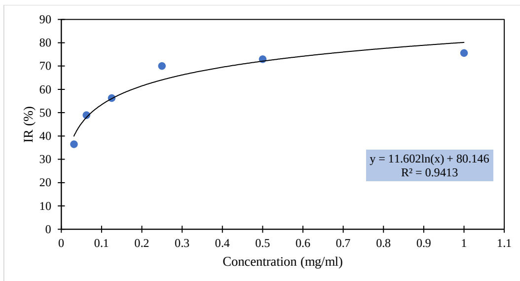
Figure 5. IC 50 for petroleum ether fraction against L.donovani
