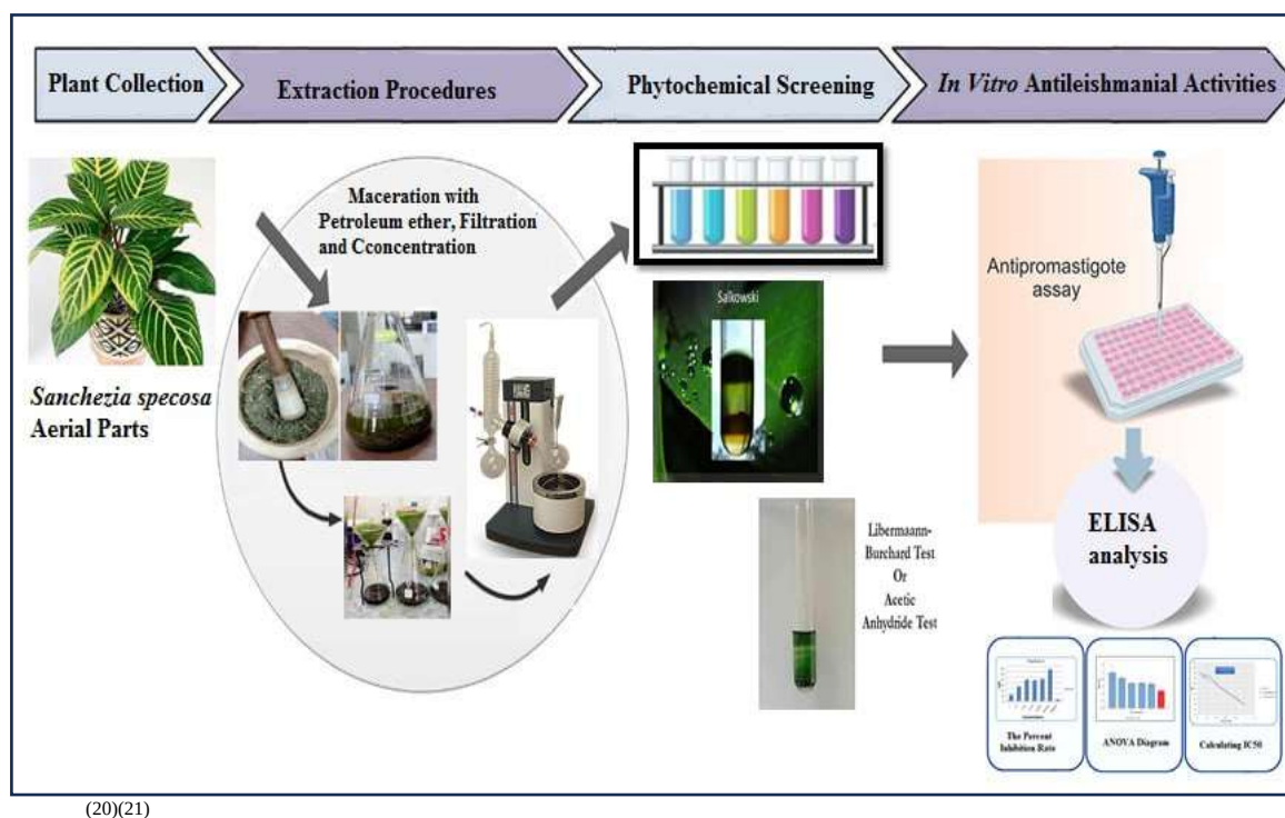
Figure 2. General scheme of Iraqi Sanchezia speciosa extraction, phytochemical identification
