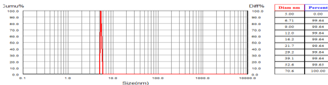
Figure (9) The particle size distribution for NF1.
