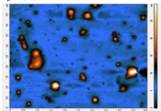
Figure (10) The AFM image of NF1 where scanning area is 5 µm * 5 µm.
